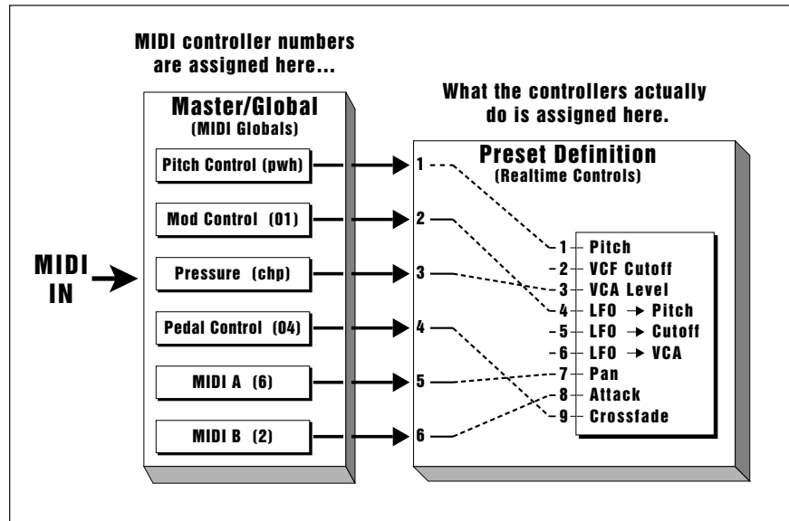
MIDI continuous controller numbers are matched to your keyboard in the MIDI submodule. The Realtime Controls submodule programs what these controllers actually do.
