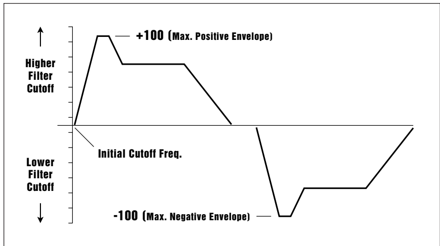
The filter cutoff frequency can be modulated with a positive or negative envelope amount.
